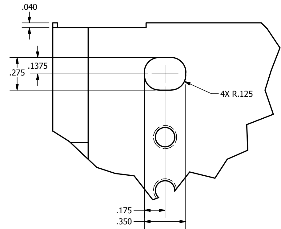
DETAIL A SLOT - 4X
